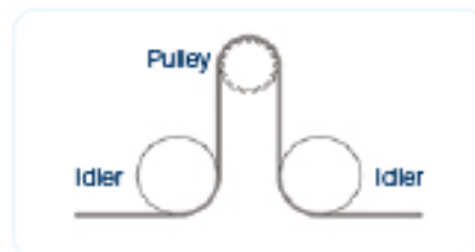
Flat idler on belt back
