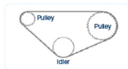
Flat idler on belt teeth
